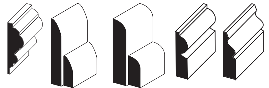
Dado Rail 18 x 58 Chamfered Skirting 14.5 x 70, 14.5 x 95, Architrave 14.5 x 45 Rounded Skirting 14.5 x 70, 14.5 x 95, Architrave 14.5 x 45 Torus Architrave 18 x 70 Ogee Architrave 18 x 58, 18 x 70 Torus Skirting 18 x 145 Ogee Skirting 18 x 145
