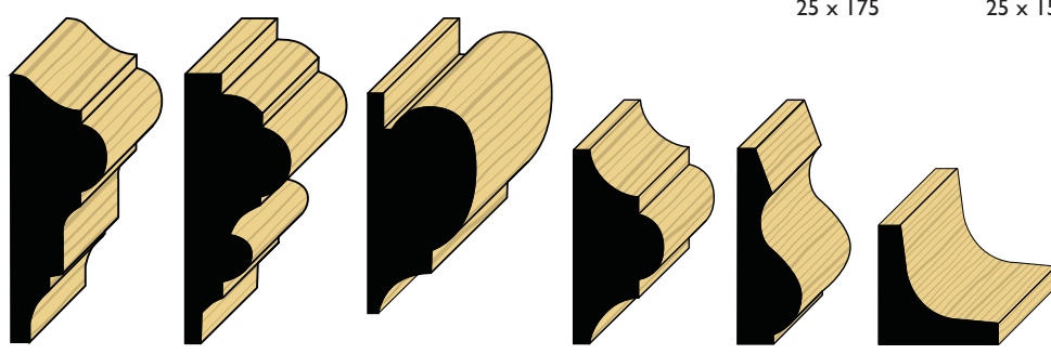
KBI Dado 25 x 63 KB2 Dado 25 x 63 KB3 Picture Rail 25 x 50 Astragal 19 x 38 Panel Mould 13 x 25, 16 x 38 Scotia 25 x 25, 38 x 38
