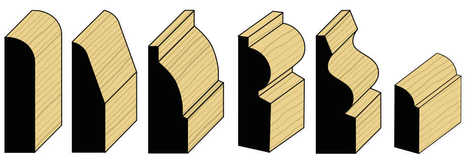
Rounded 19 x 50 Chamfered 19 x 50 Ovolo 25 x 63 Torus 25 x 75 Ogee 25 x 50, 25 x 63, 25 x 75 Ovolo Door Stop 16 x 38
